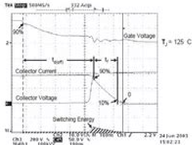
Figure 19. Turn-off Switching Waveforms and Definitions
