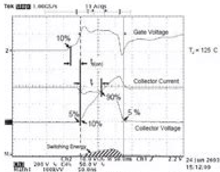
Figure 18. Turn-on Switching Waveforms and Definitions
