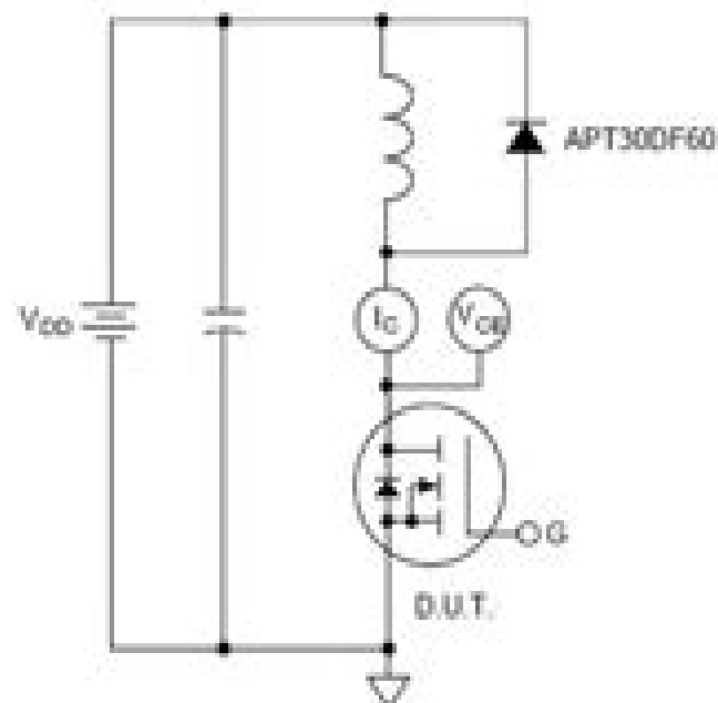
Figure 20. Inductive Switching Test Circuit
