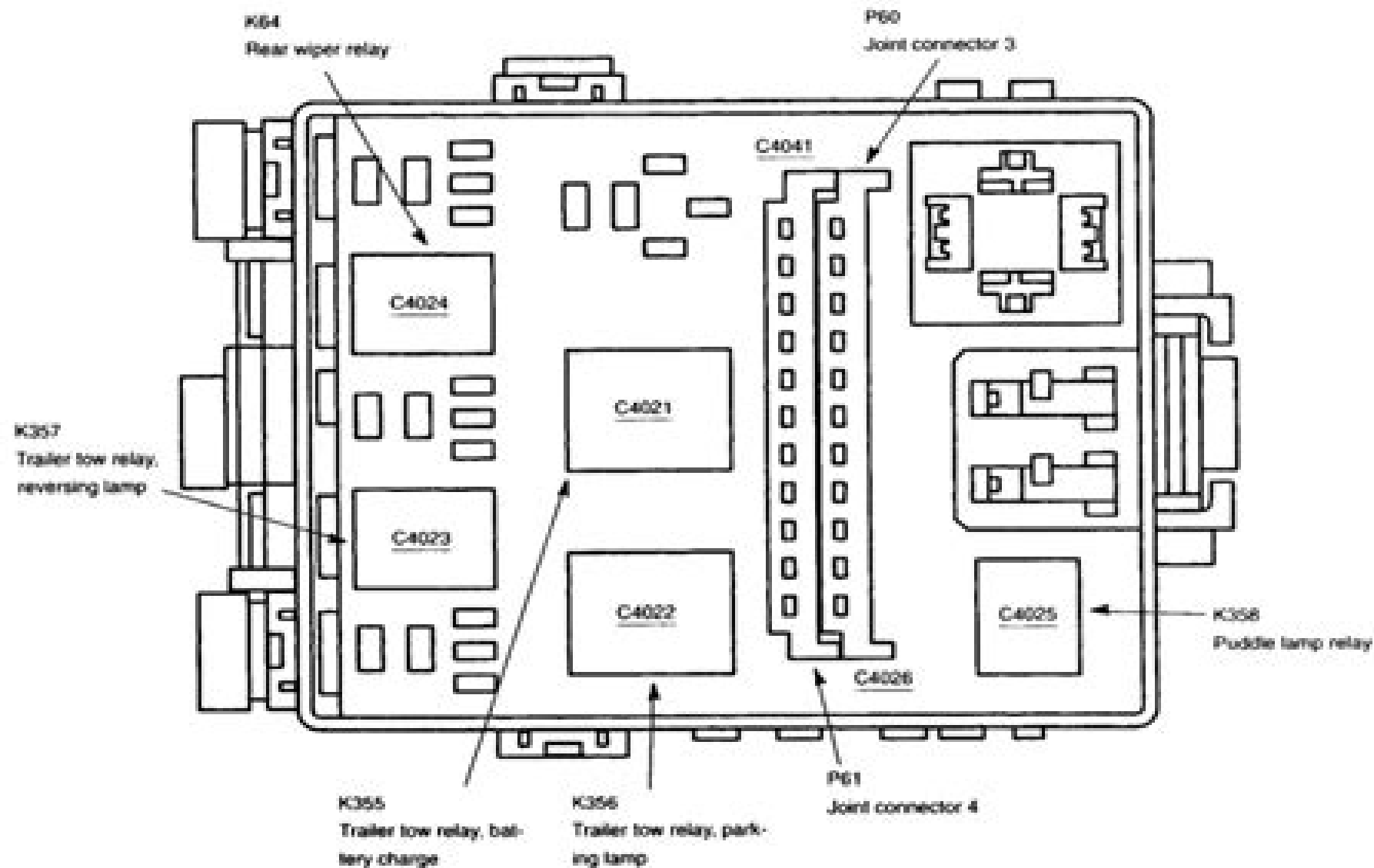
Fig 3: Identifying Auxiliary Junction Box, Rear, Relays
