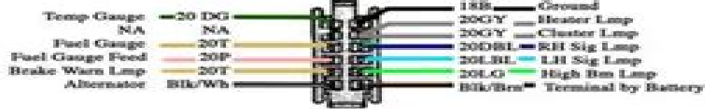
Instrument Cluster Connection With Gauges
