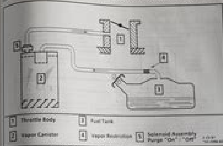
Figure C-3 K Evaporative Emission Control System Schematic
