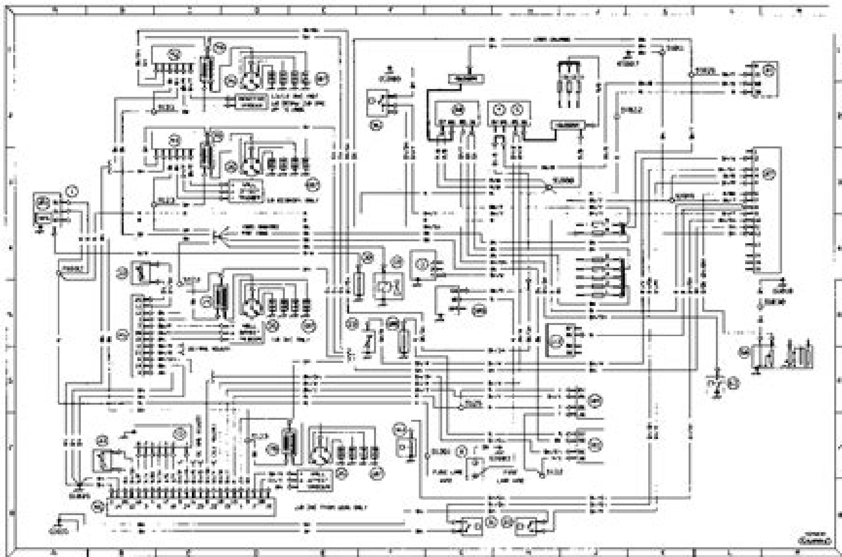
Diagram 1. Starting, charging and ignition (except fuel injection). Models up to 1967
