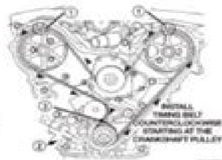
Fig. 76 Timing Belt—Installation
