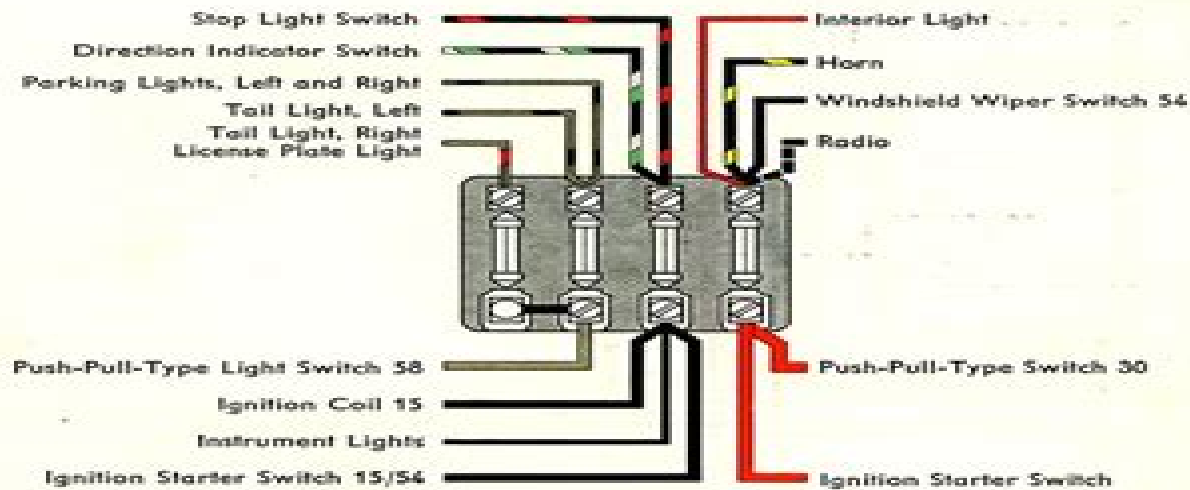
Fuse box on the back of the instrument panel
