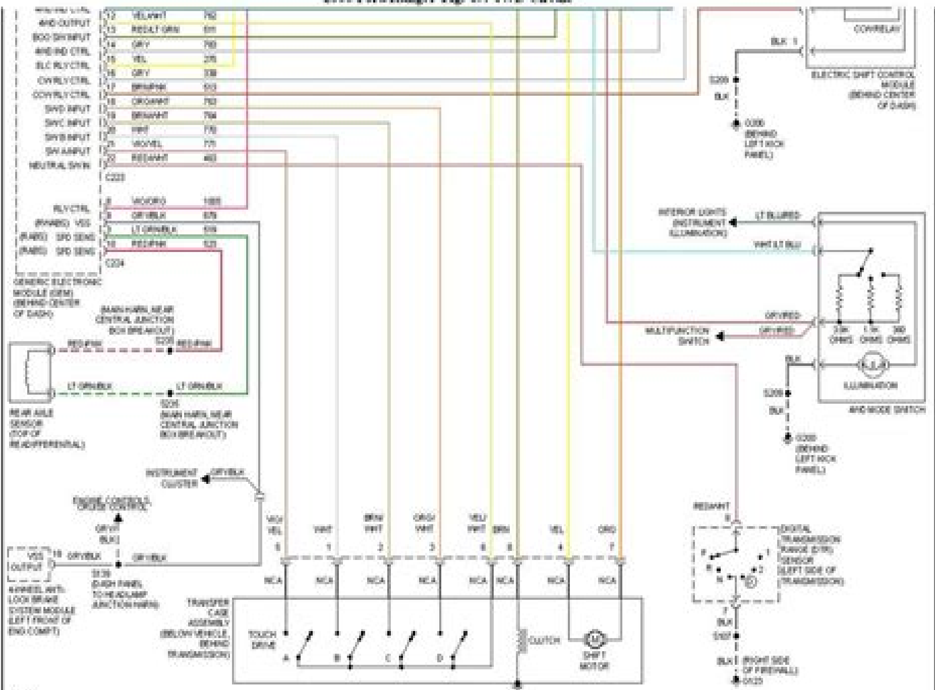
2000 Ford Ranger-Fig. 49: 4WD Circuit
