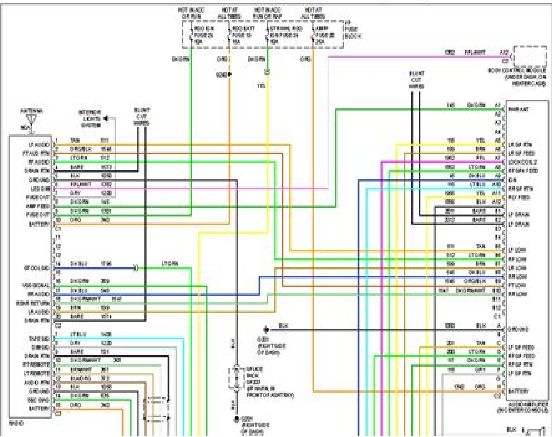
2001 GMC Jimmy - Fig. 48: Radio Circuits, W/ Amplifier
