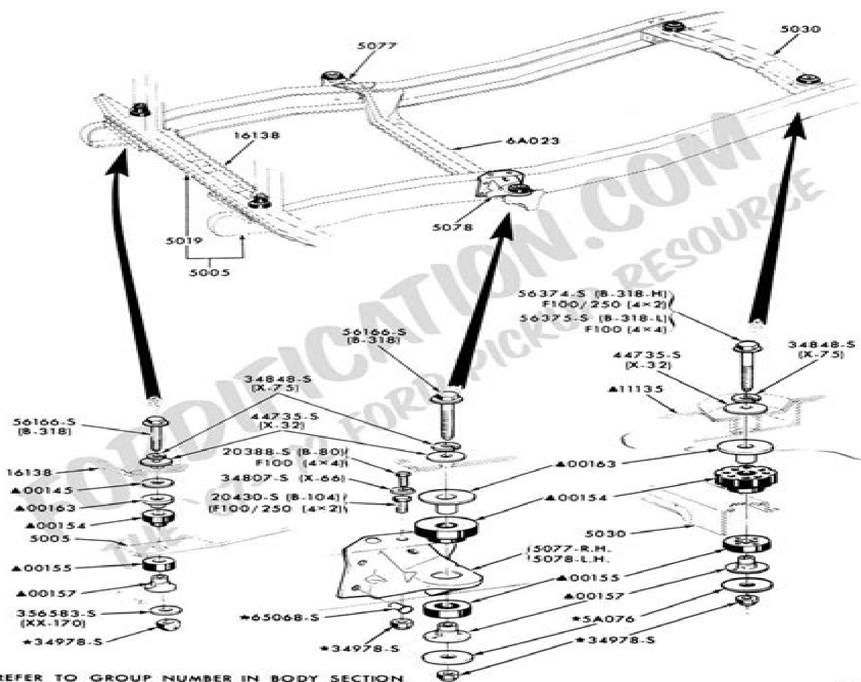
FRAME FRONT END and BODY MOUNT PARTS 1964/72 F100/250 (4 x 2), F100 (4 x 4)
