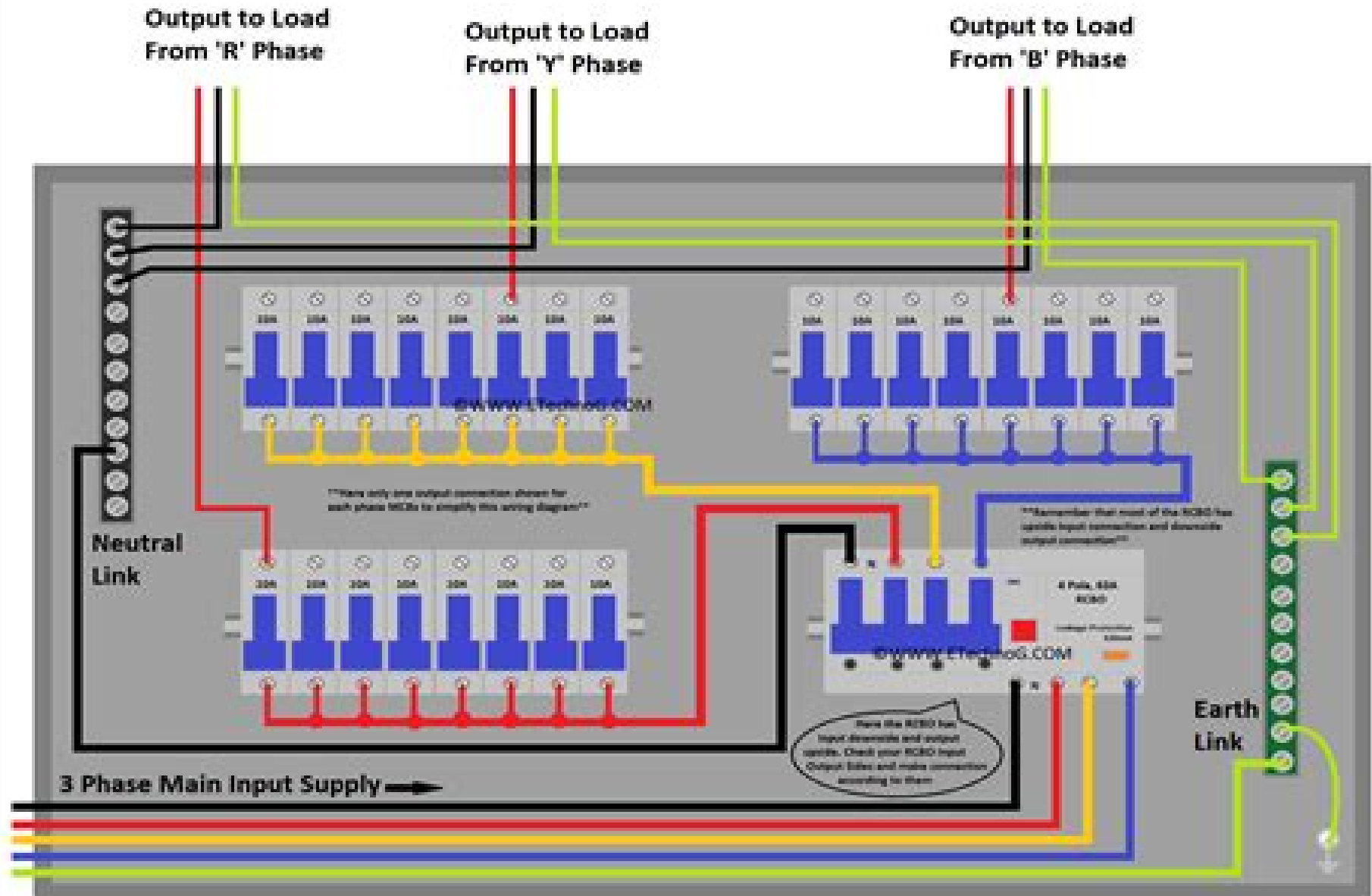
3 Phase to Single Phase Distribution Board Wiring Diagram and Connection Procedure
