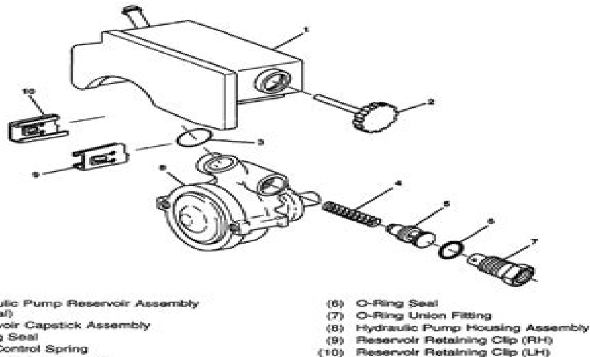
Fig. 5: Exploded View Of Power Steering Pump Assembly-CB Series Courtesy of GENERAL MOTORS CORP.
