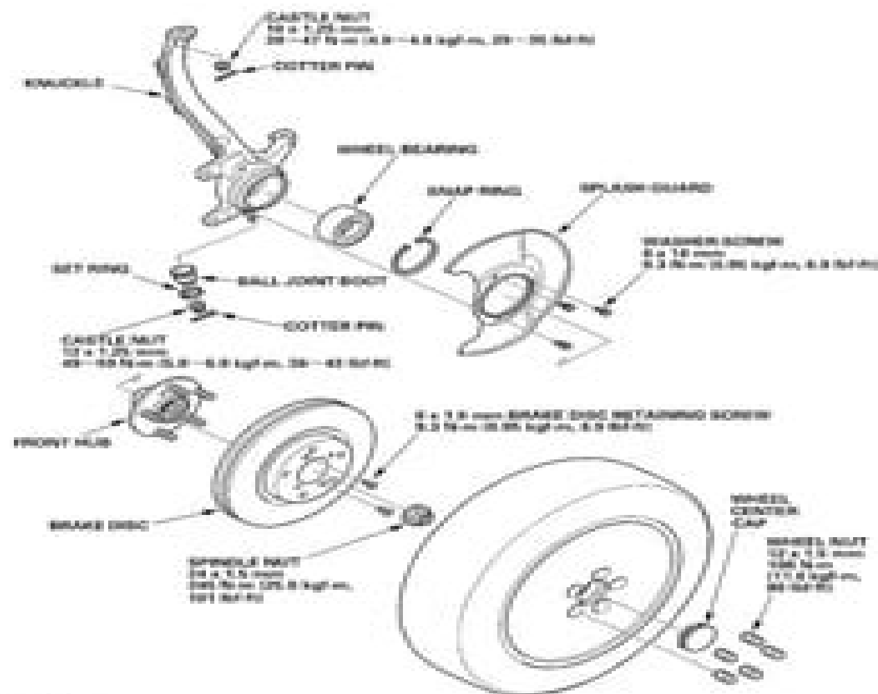
Fig. 7: Exploded View Of Knuckle & Hub Courtesy of AMERICAN HONDA MOTOR CO., INC.
