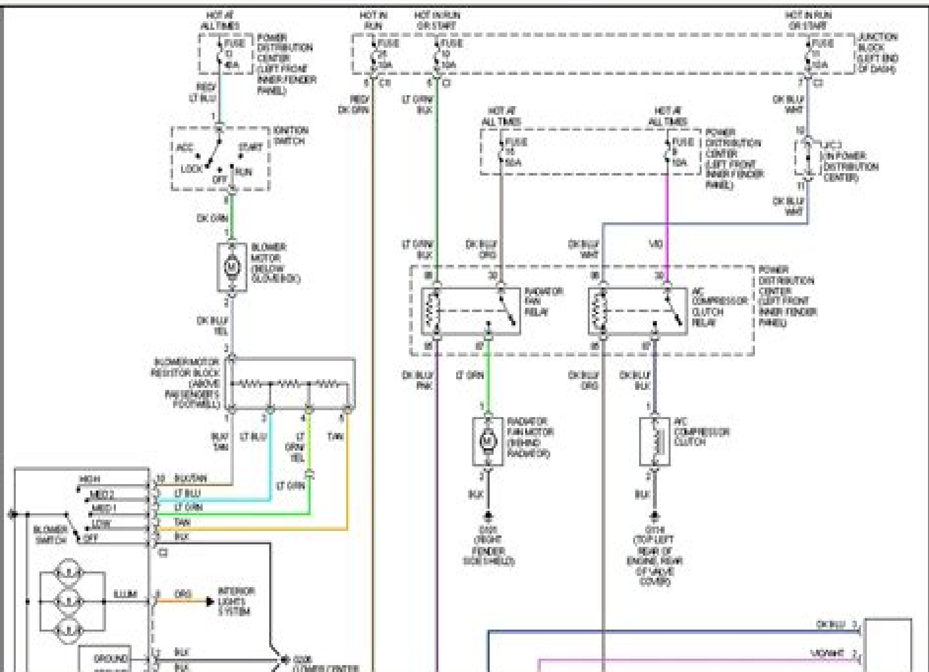
Fig. 25 Manual A/C Heater System Wiring Diagram (2001 Dakota)
