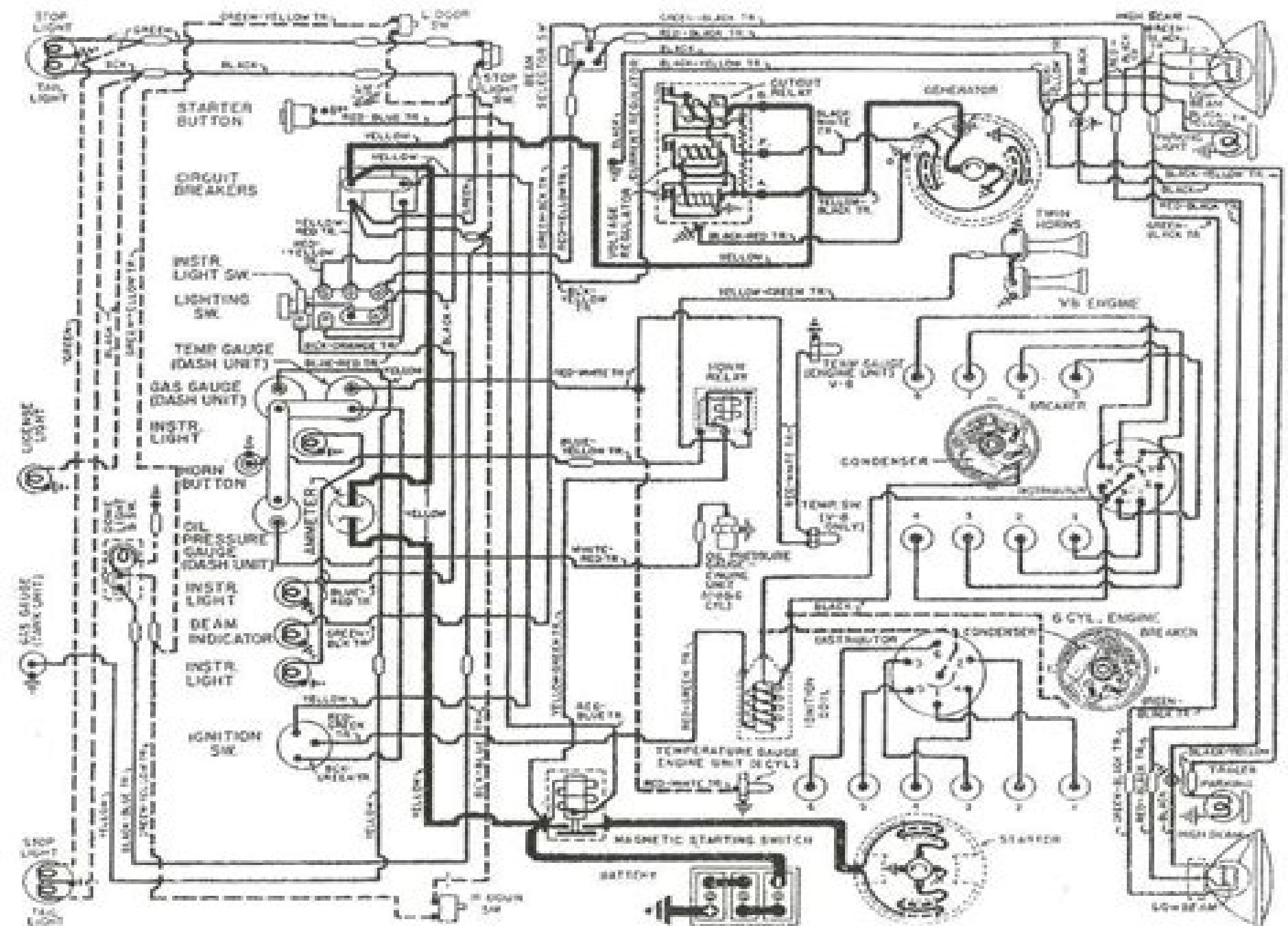
1951-1952 FORD TRUCKS LIGHT DUTY F-1, F-2, F-3 & HEAVY DUTY F-4, F-5 & F-6 WIRING DIAGRAM
