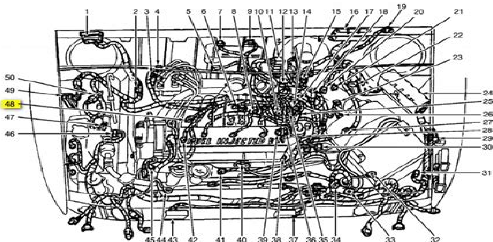
3.8L ENGINE
