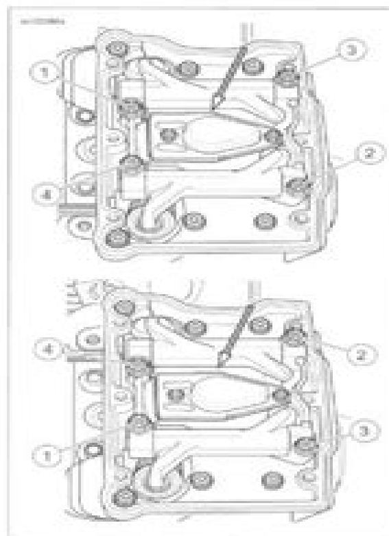
Figure 3-19. Rocker Arm Support Tightening Sequence
