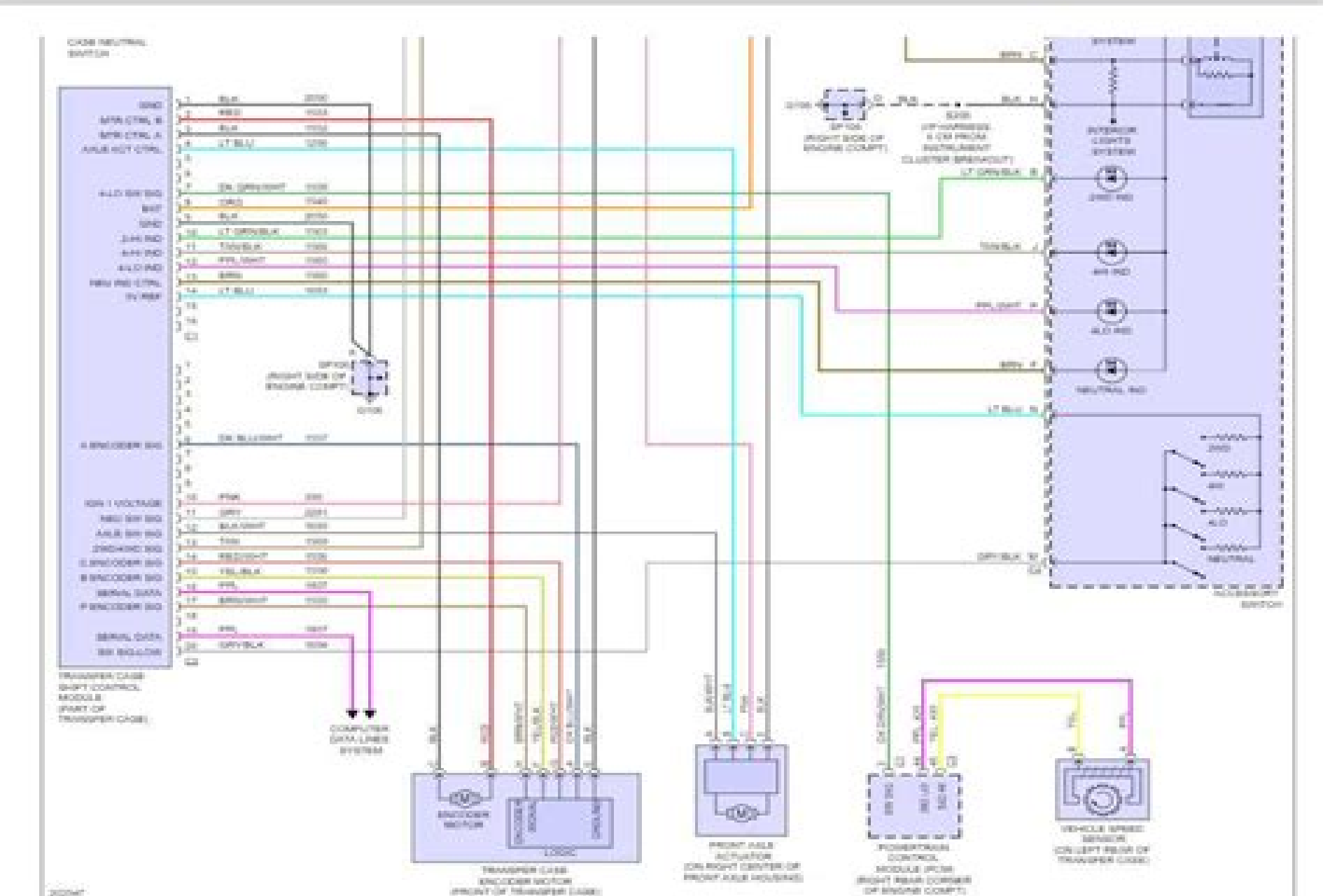
Fig 2: Transfer Case Circuit
