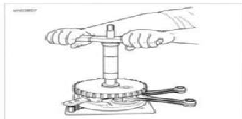
Figure 3-136. Press Inner Race onto Sprocket Shaft: Operation
