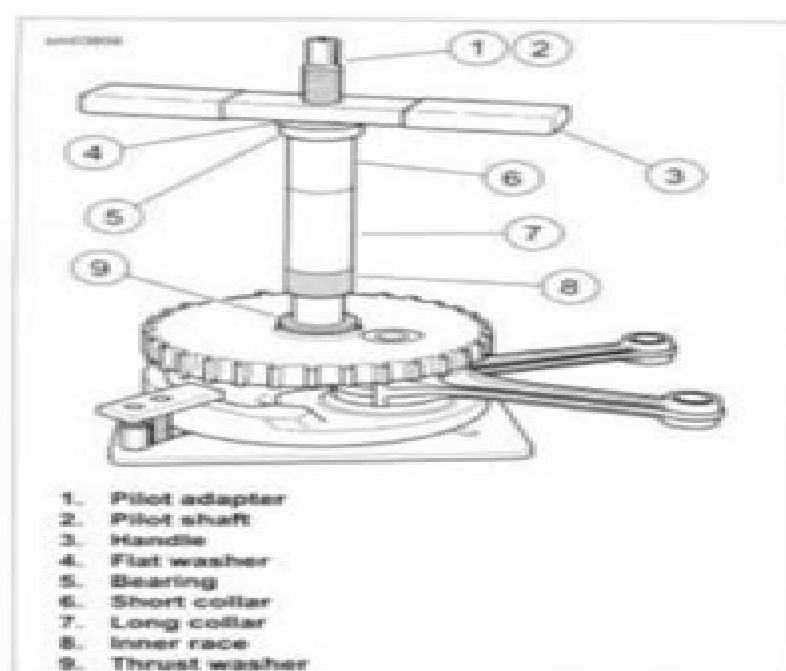
Figure 3-135. Press Inner Race onto Sprocket Shaft: Setup
