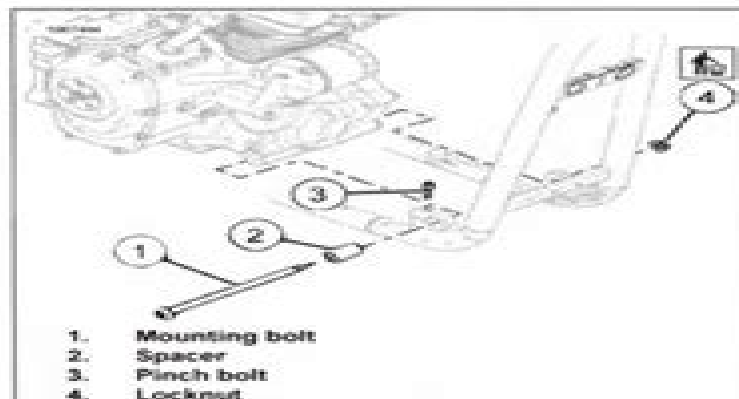
Figure 4-14. Lower Front engine Mount
