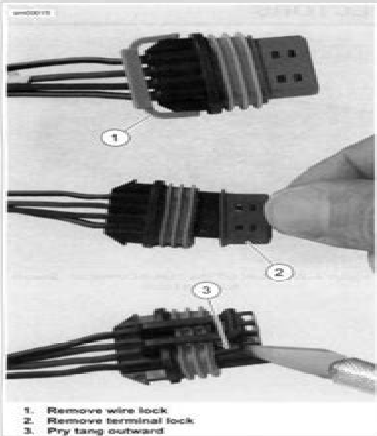
Figure A-21. Delphi GT 150 Sealed Connector: Removing Socket Terminals
