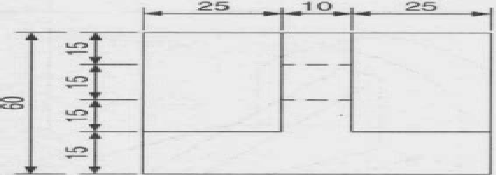
Front View
