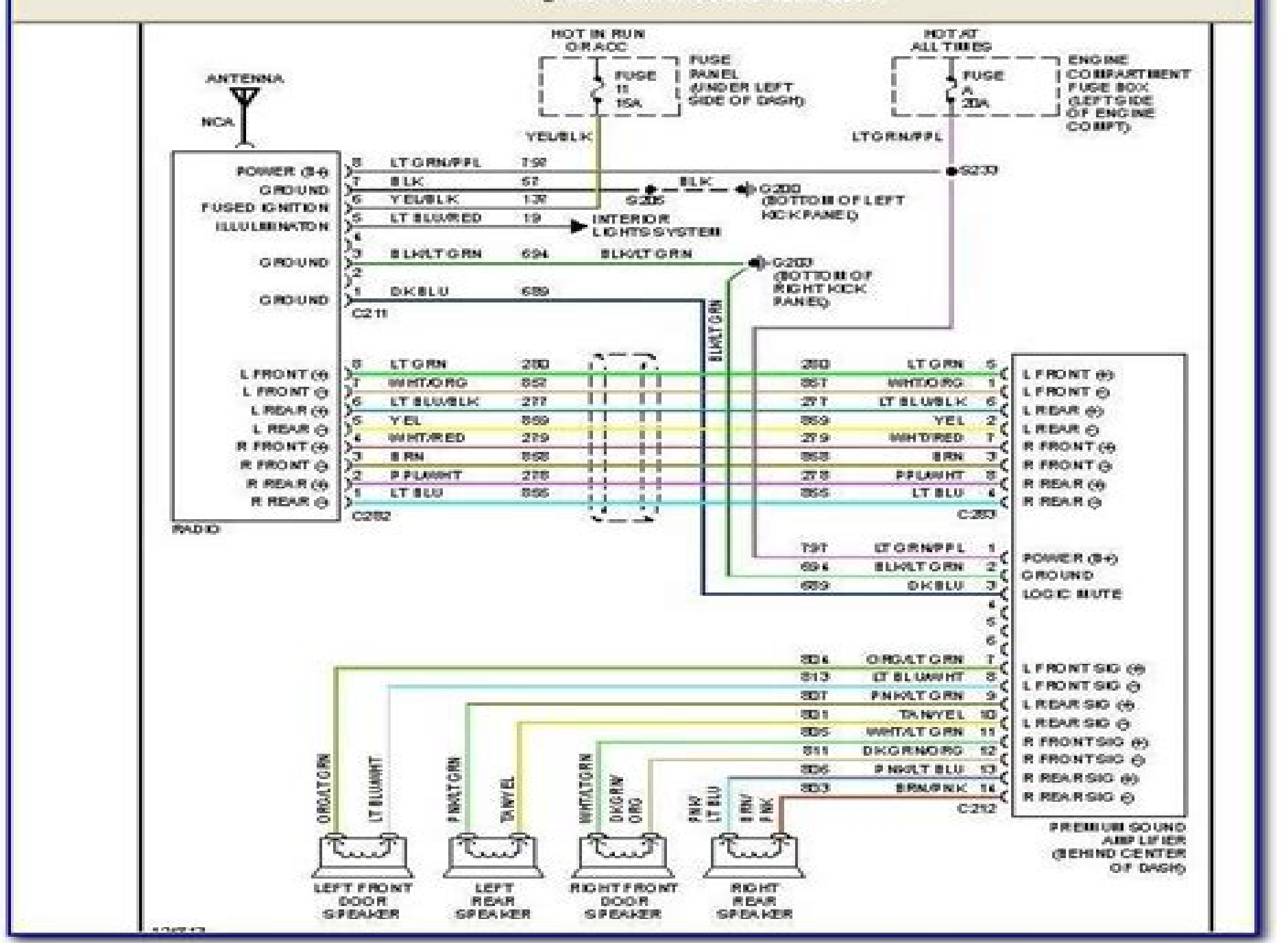
Fig. 58: Premium Sound Radio Circuit
