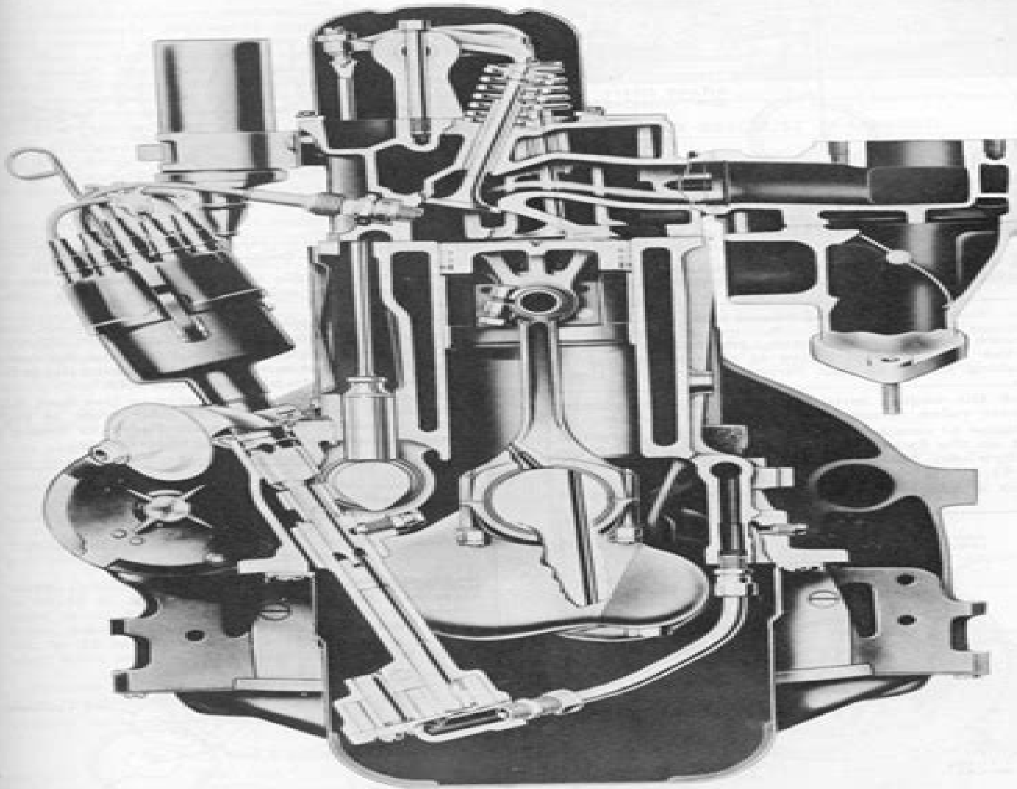
Fig. 1—Engine Cross Section
