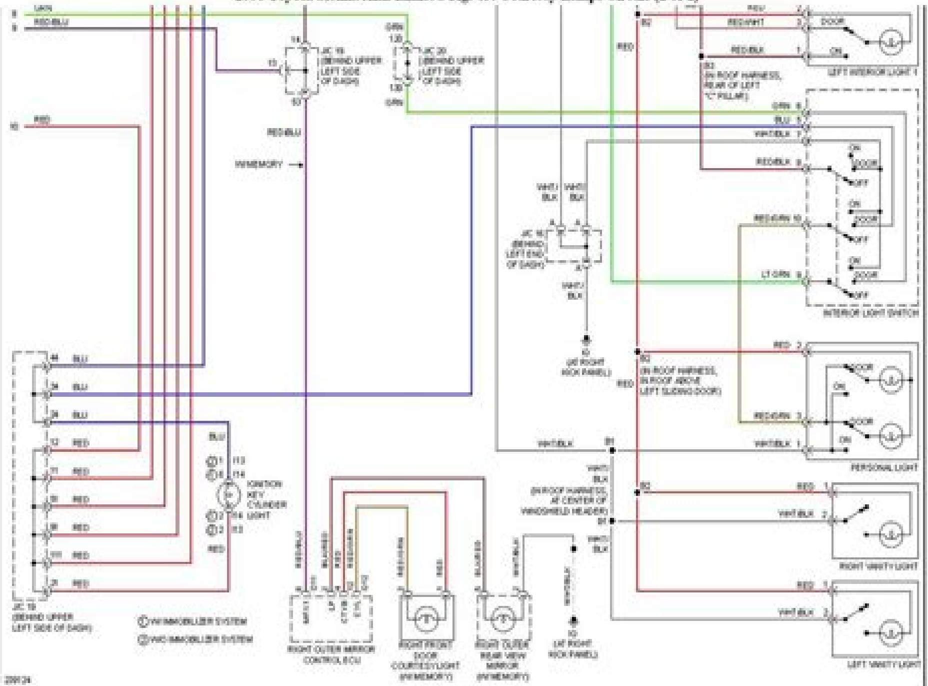
2004 Toyota Sienna XLE Limited Fig. 43: Courtesy Lamps Circuit (2 of 2)
