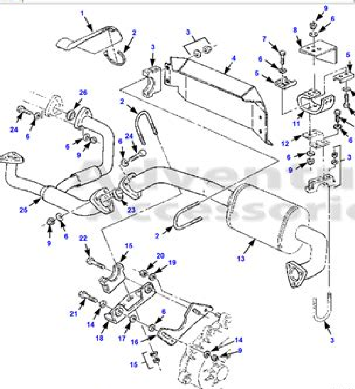
Muffler, Exhaust Pipes and Related Parts (1994) (Figure 1 of 2)
