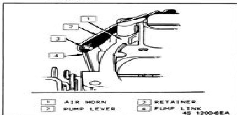
Figure 91 Removing Pump Link From Lever (E4ME)
