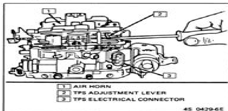
Figure 93 Installing Air Horn
