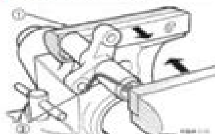
Fig. 98 Compressing Timing Belt Tensioner
