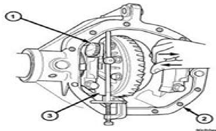
Fig. 17 RECORD DIAL INDICATOR
