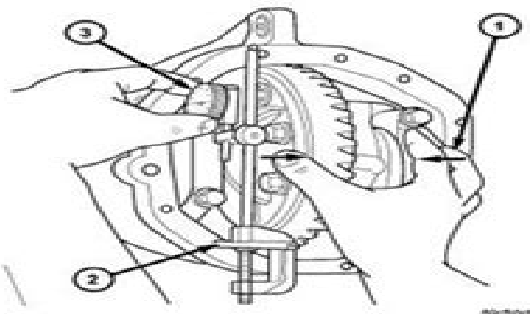
Fig. 16 ZERO DIAL INDICATOR
