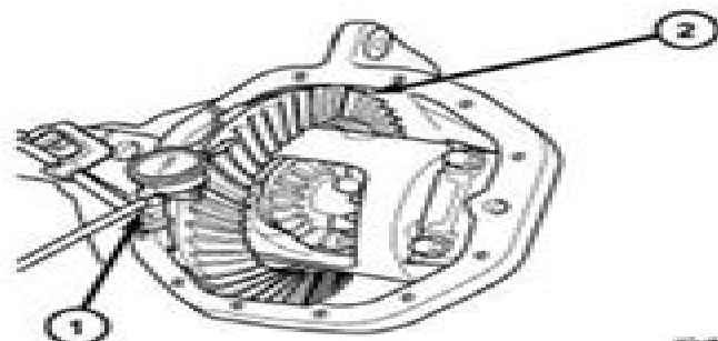
Fig. 18 RING GEAR BACKLASH
