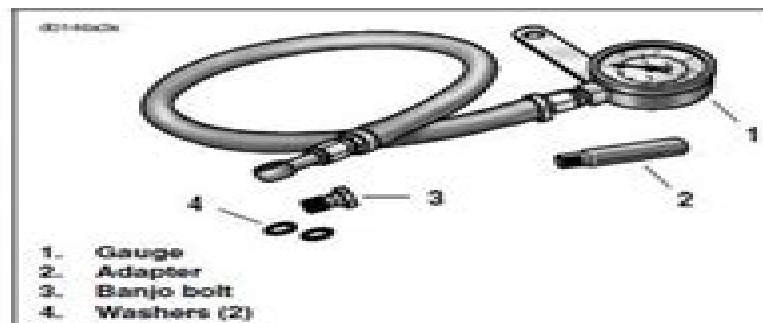
Figure 3-14. Oil Pressure Gauge
