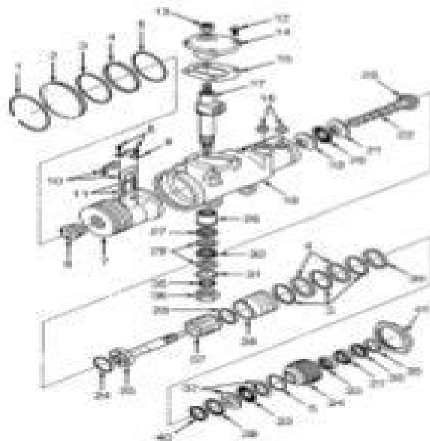
Fig. 1. Exploded View Of Power Steering Gear Courtesy of GENERAL MOTORS CORP.
