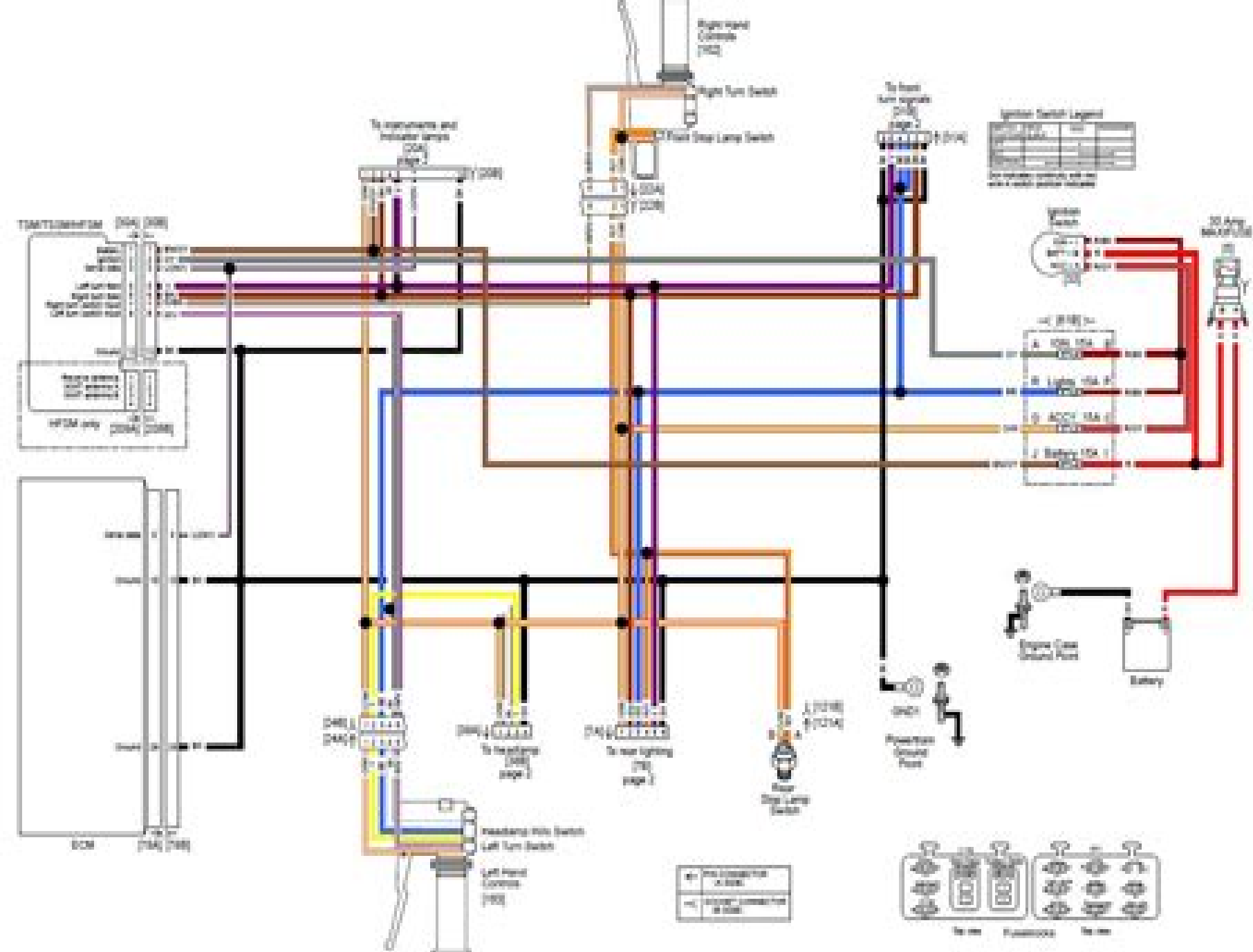
Figure B-7. 2008 SPORTSTER DOM and INT MODELS, LIGHTS (1 of 2) (DL)
