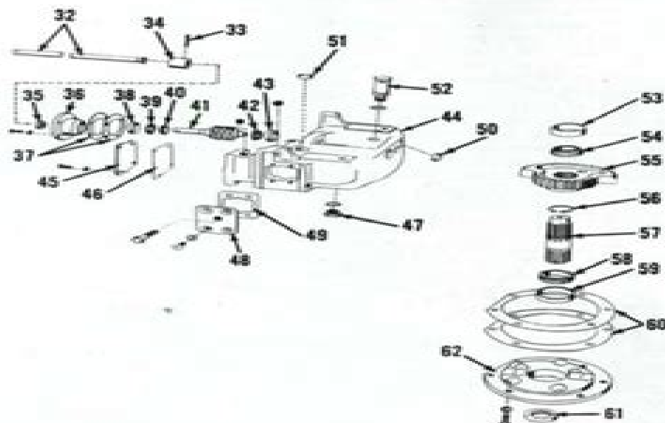
Fig. 7—Exploded view of manual steering front support and associated parts. Shims (37) are available in 0.005 veltum or steel; shims (48) are available in either veltum or steel, veltum being 0.005 and steel 0.010 thick.
