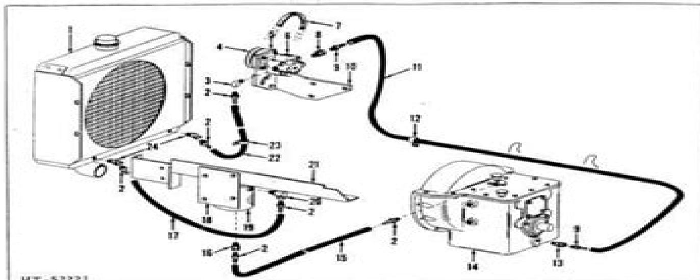
TRANSMISSION & CONNECTIONS (OIL CLUTCH) F-FL 30-40-50 CATALOG NO. 4799098
