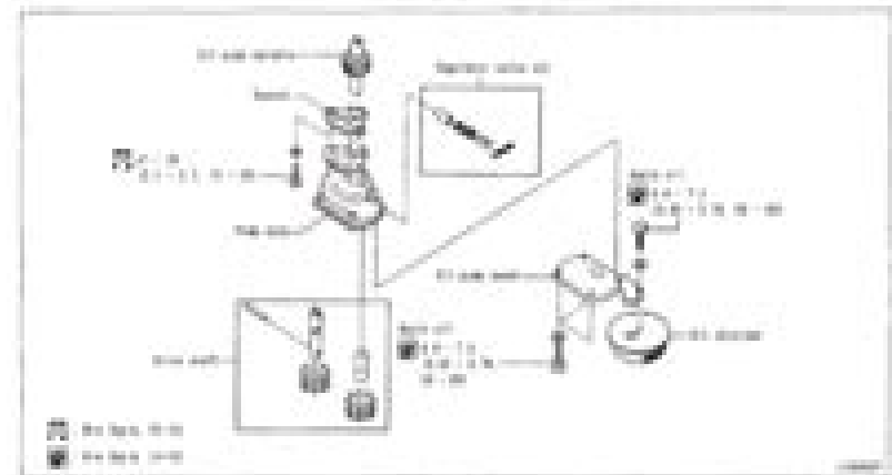
Oil Pump component parts location
