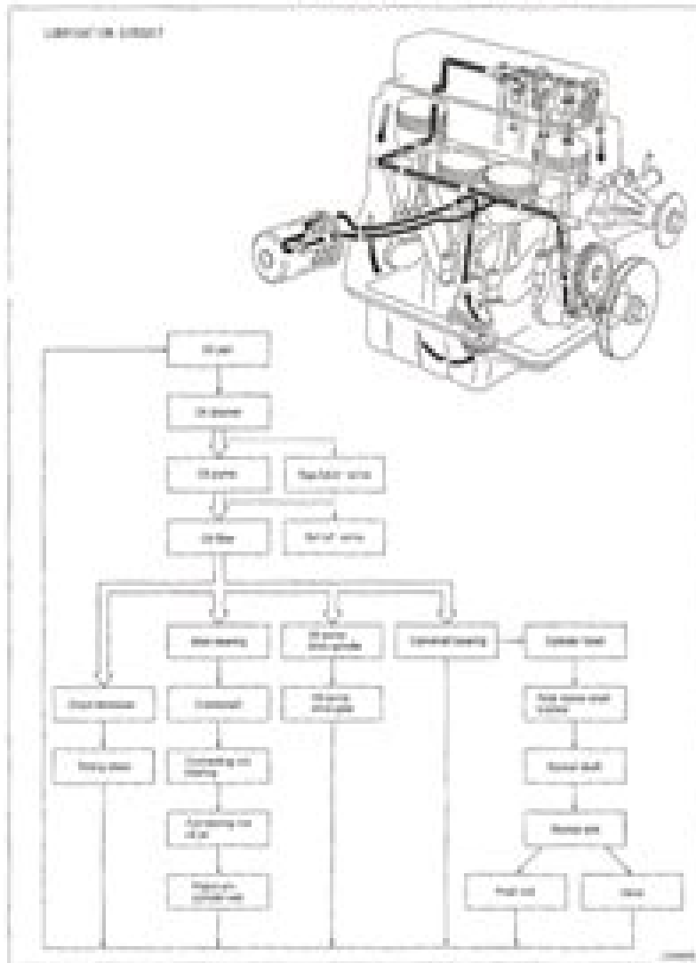
Luteration Schematic Diagram
