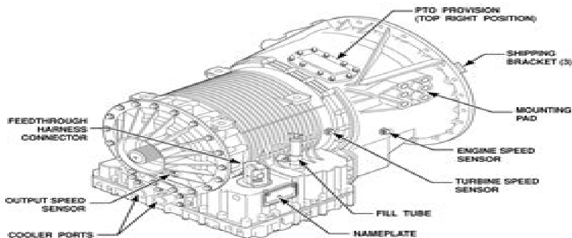
Figure 1-1. 4000 Product Family Transmission With PTO Provision (Except 4700 and 4800 Models)—Right-Rear View
