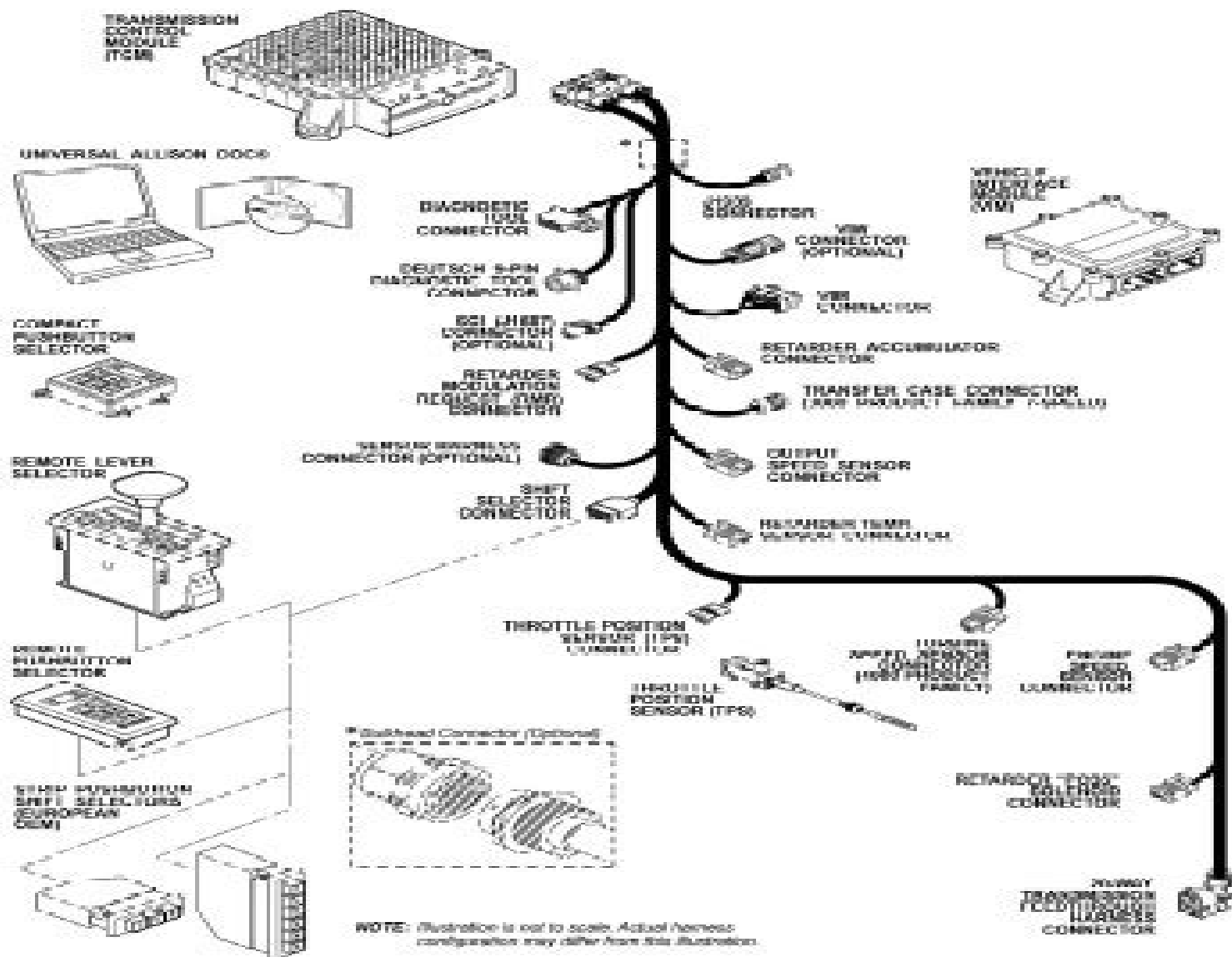
Figure 2–1. Typical 4th Generation Electronic Controls External Wiring Harnesses
