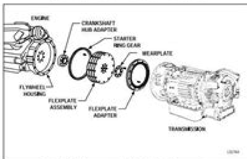
Figure 4-3. Arrangement of Adaptation Components
