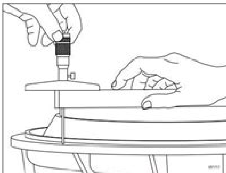
Figure 4-2. Converter Axial Location Measurement
