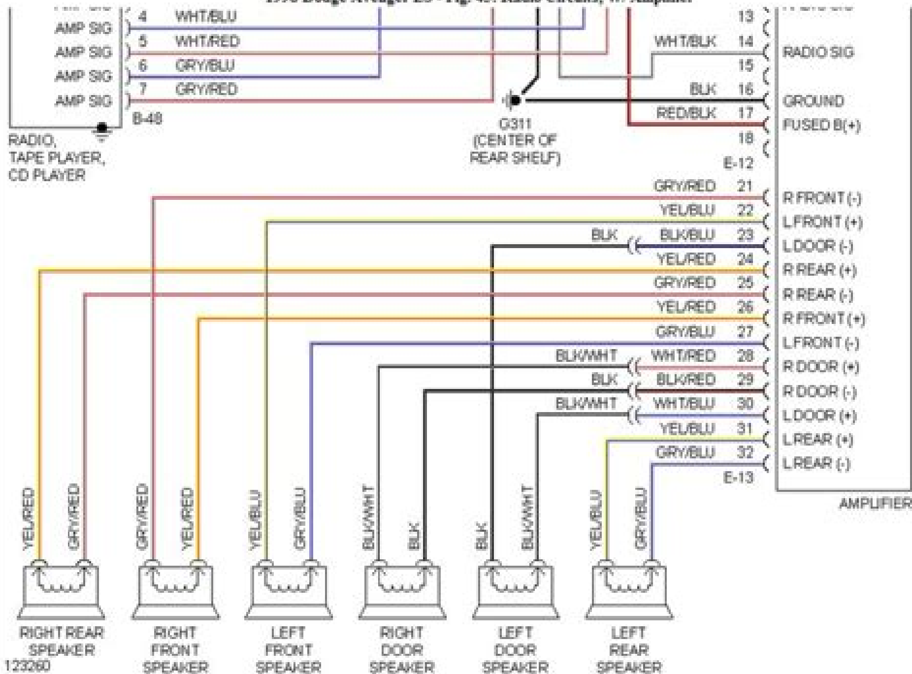
1998 Dodge Avenger ES - Fig. 45: Radio Circuits, W/ Amplifier
