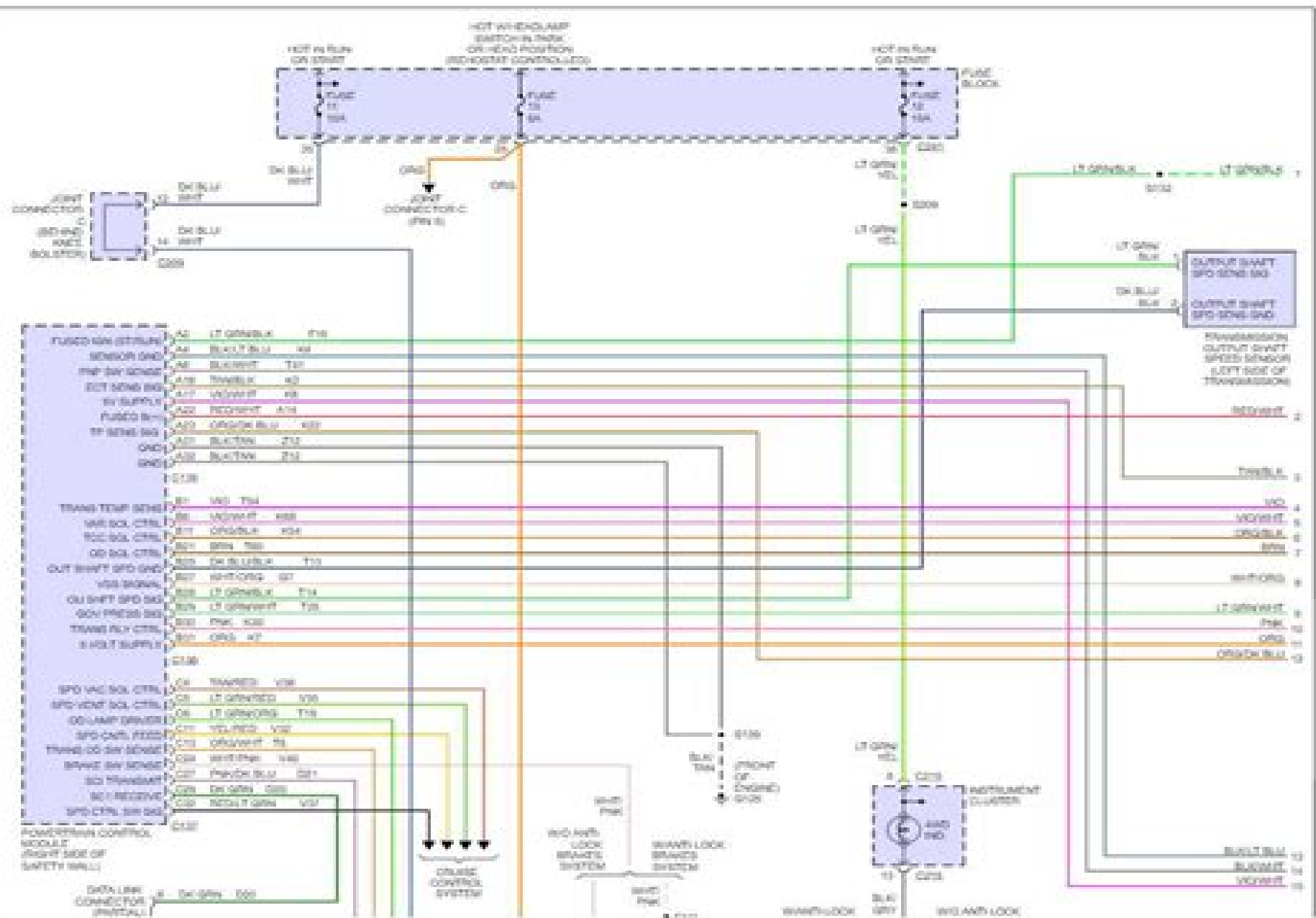
Fig 3: 5.2L Transmission Circuit (1 of 2)
