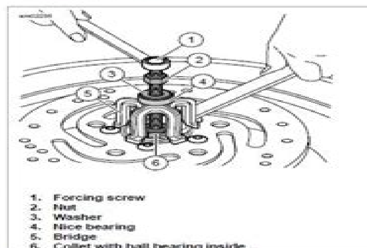
Figure 2-12. Removal Tool
