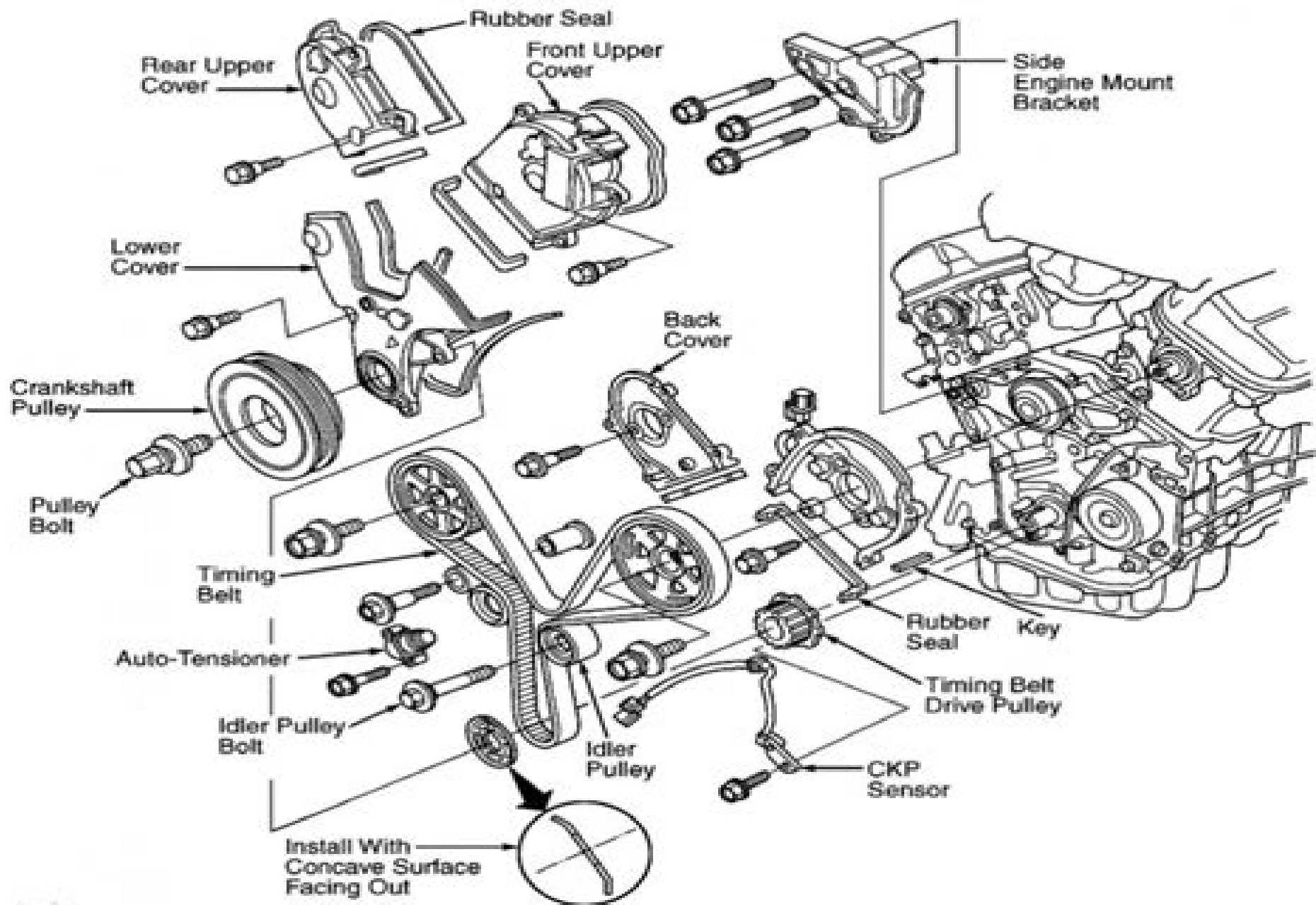
Fig. 2: Exploded View Of Timing Belt & Components Courtesy of AMERICAN HONDA MOTOR CO., INC.
