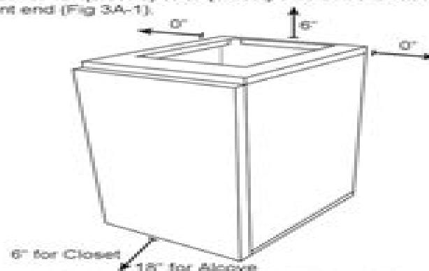
Fig 3A-1. Minimum Clearance for Electric Furnace
