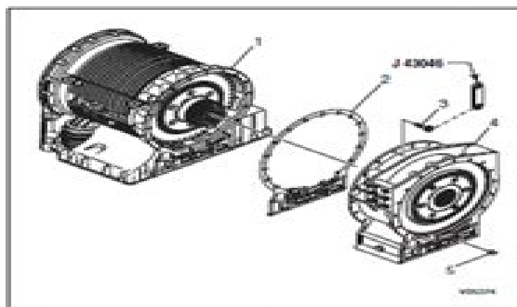
Figure 4-13. Removal of C6 Adapter Housing Module (4700 and 4800 Models)
