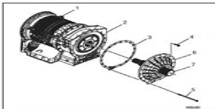
Figure 4-11. Removal of Rear Cover and Output Shaft Module
