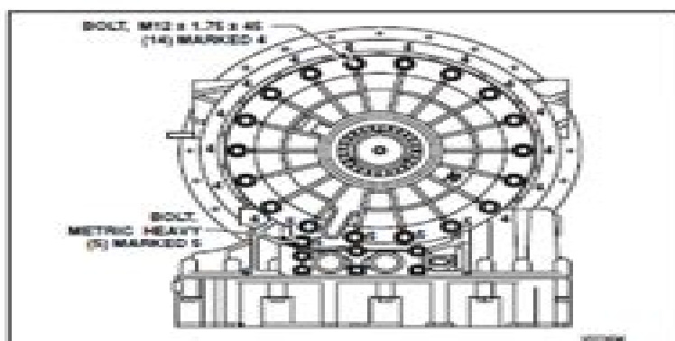
Figure 4-12. Rear Cover and Output Shaft Module Bolts
