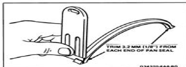
Fig. 33 Trimming Oil Pan Seals
