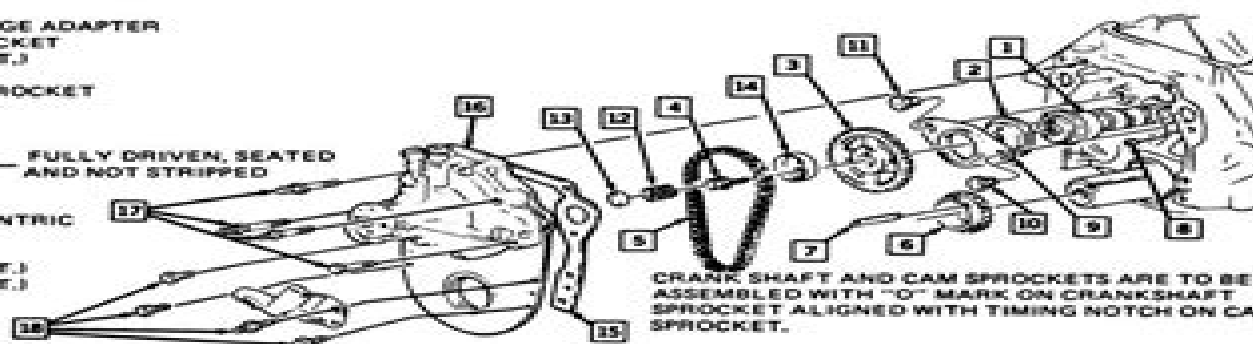
Fig. 32 Front of Engine
