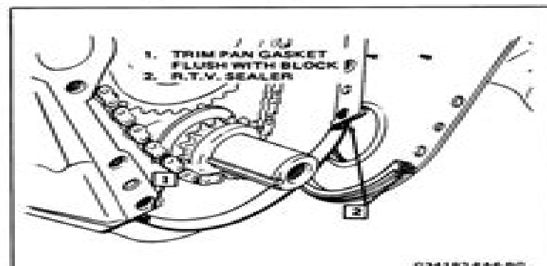
Fig. 34 Applying RTV Sealer and Trimming Oil Pan Gasket
