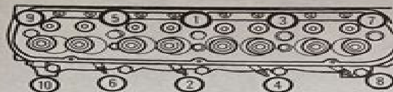
9.22 Cylinder head bolt tightening sequence
