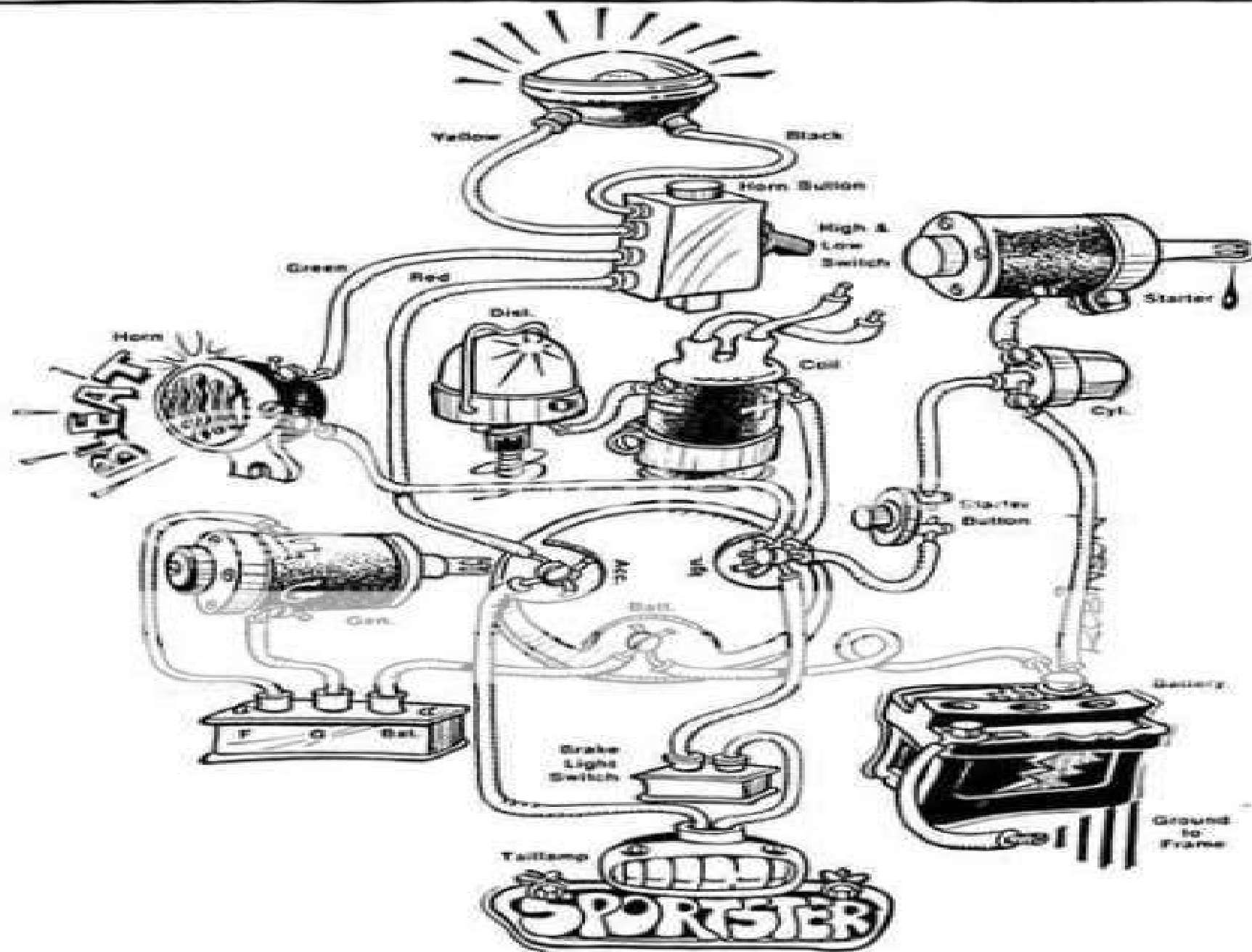
Wiring Diagram for an Electric-Start Sportster
