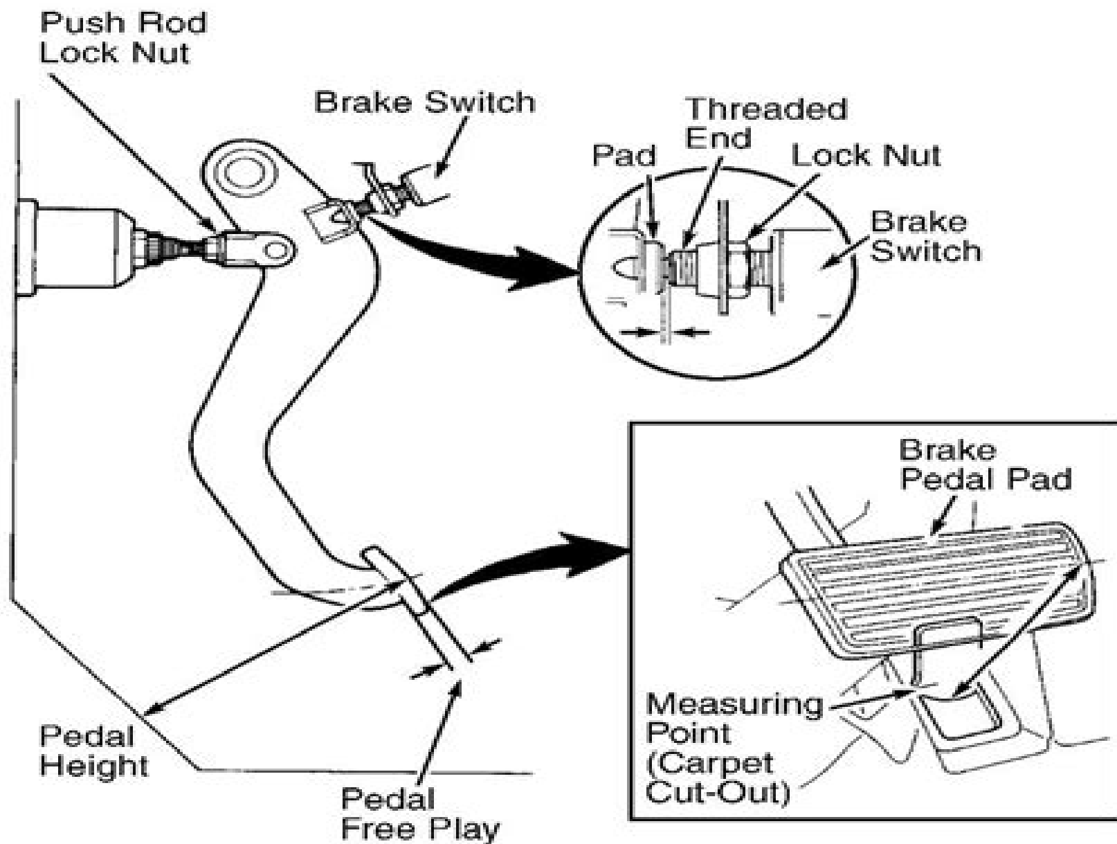
Fig. 2: Adjusting Brake Pedal Height & Free Play Courtesy of AMERICAN HONDA MOTOR CO., INC.
