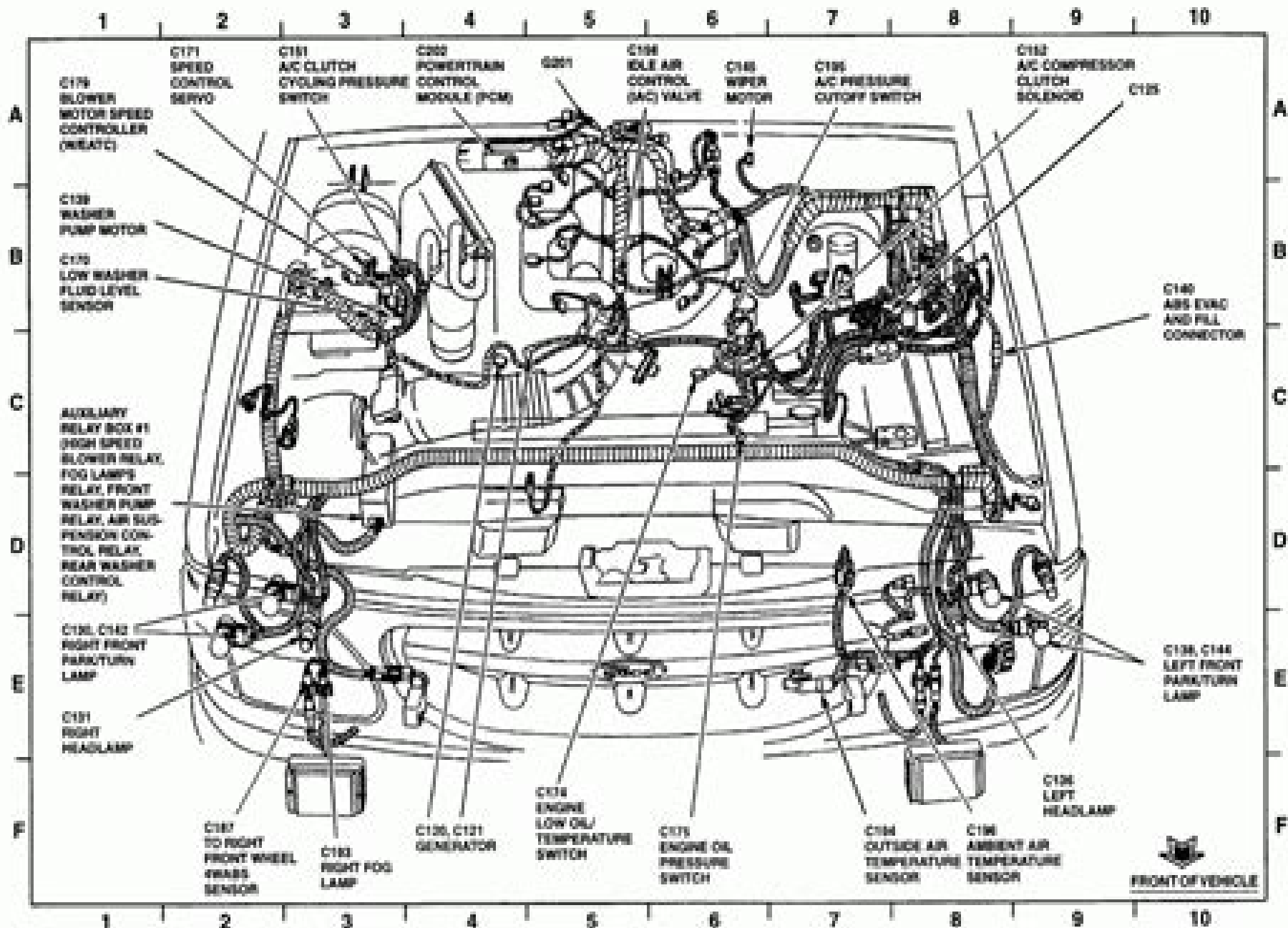
4.0L SOHC ENGINE (1 OF 3)
