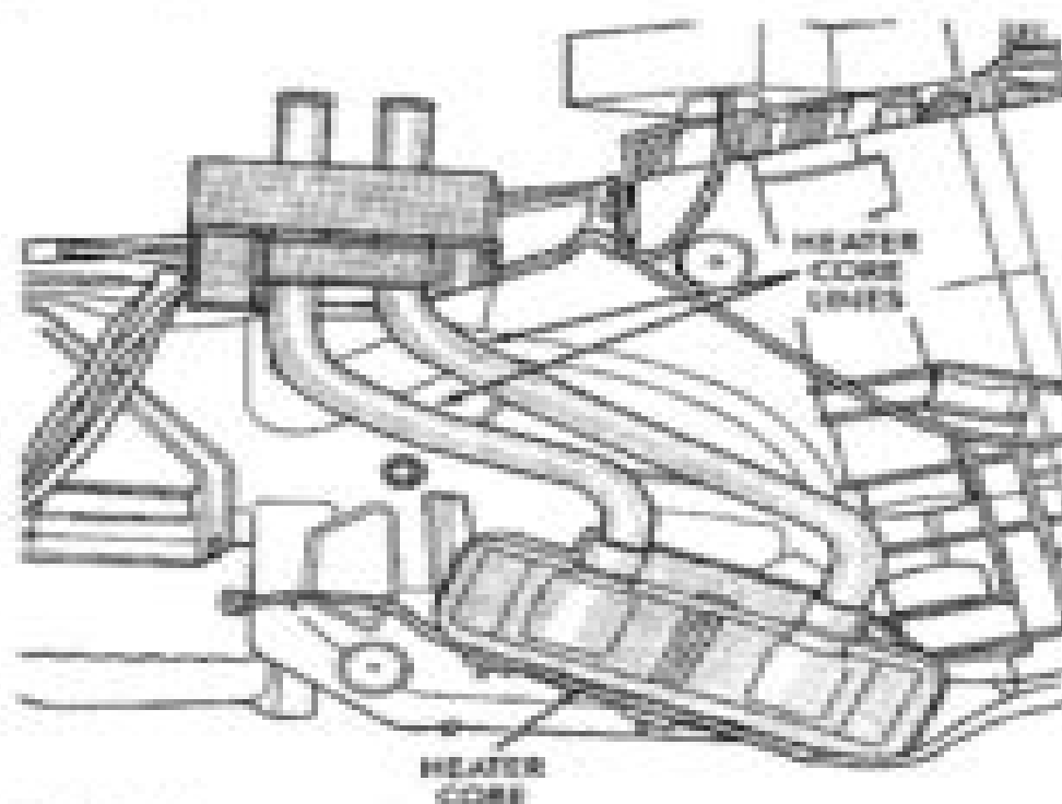
Fig. 6: Identifying Heater Core Location
